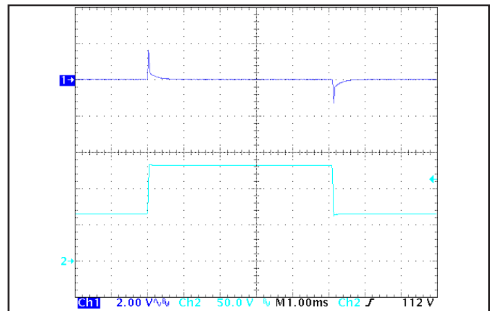
Figure 6: Output voltage response to step-change in input voltage (1000 V/ms). Load cap: 100 μF, electrolytic output capacitance. Ch 1: V out (2 V/div), Ch 2: V in (50 V/div).
