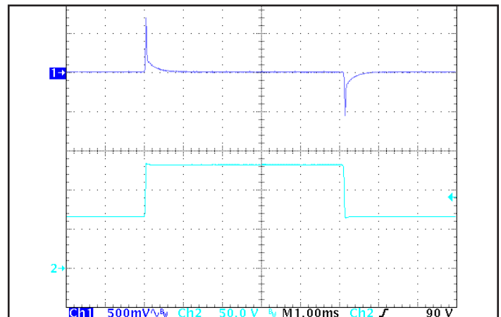
Figure 6: Output voltage response to step-change in input voltage (1000 V/ms). Load cap: 100 µF, electrolytic output capacitance. Ch 1: V out (500 mV/div), Ch 2: V in (50 V/div).
