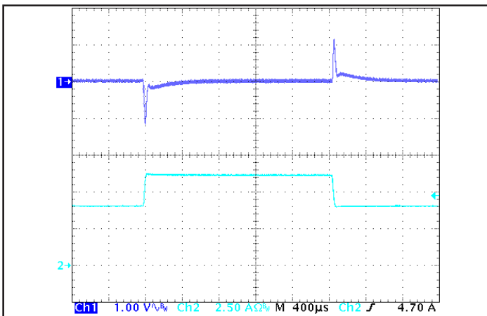
Figure 5: Output voltage response to step-change in load current (50% -75% -50% of I out (max); dI/dt = 0.1 A/μs). Load cap: 1 μF ceramic capacitor. Ch 1: V out (1 V/div), Ch 2: I out (2.5 A/div).
