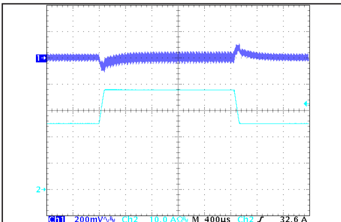
Figure 5: Output voltage response to step-change in load current (50% -75% -50% of I out (max); dI/dt = 0.1 A/μs). Load cap: 15 μF Tantalum + 1 μF ceramic capacitor. Ch 1: V out (200 mV/div), Ch 2: I out (10 A/div).
