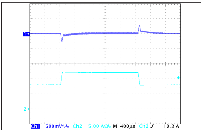
Figure 5: Output voltage response to step-change in load current (50% -75% -50% of I out(max) ; dI/dt = 0.1 A/µs). Load cap: 15 µF Tantalum + 1 µF ceramic capacitor. Ch 1: V out (500 mV/div), Ch 2: I out (5 A/div).
